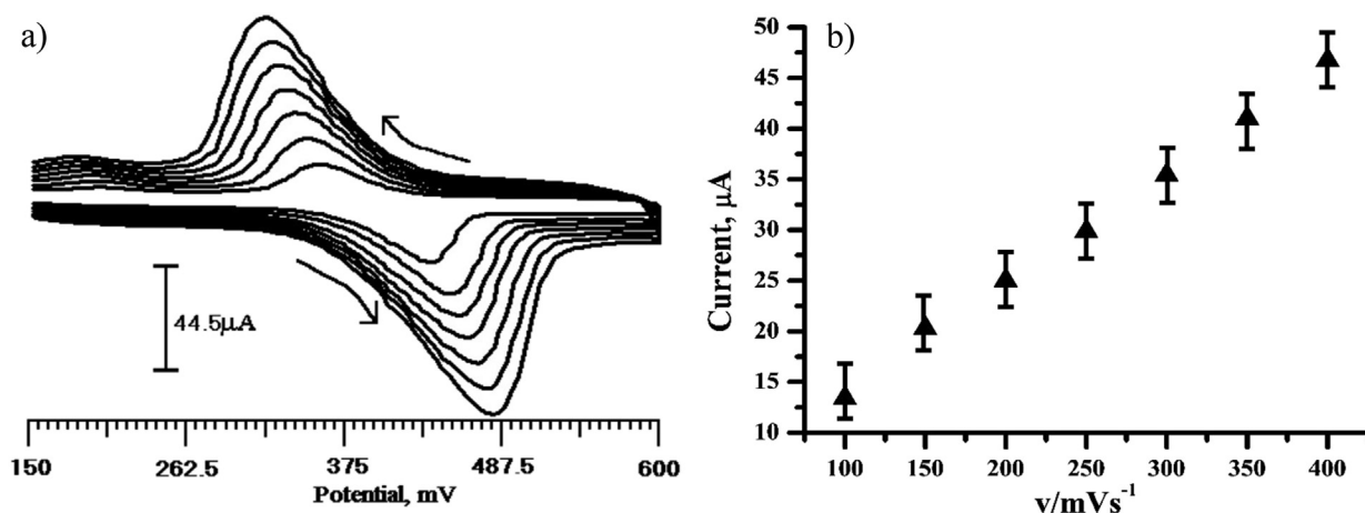
Fig. 7 – (a) Cyclic voltammograms of IC ( 1 \times 10^{-4} M) at the PGMCPe in pH 6.5 PBS at various scan rates. From: 100, 150, 200, 250, 300, 350 and 400 mV/s. (b) Plot of the peak current of IC as a function of the scan rate.
