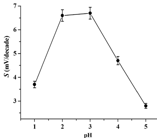
Fig. 3 – Influence of pH on the response of the proposed electrode.
