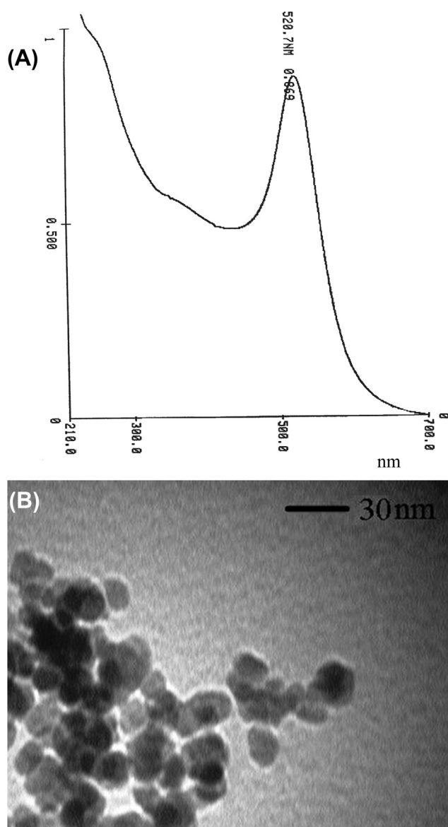
Fig. 2 – (A) UV–Vis spectrum and (B) TEM image of the prepared Au NPs. Au NP = gold nanoparticle; TEM = transmission electron microscopy; UV–Vis = ultraviolet–visible.
