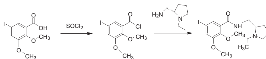
Fig. 2 – Scheme for the preparation of epidepride.
