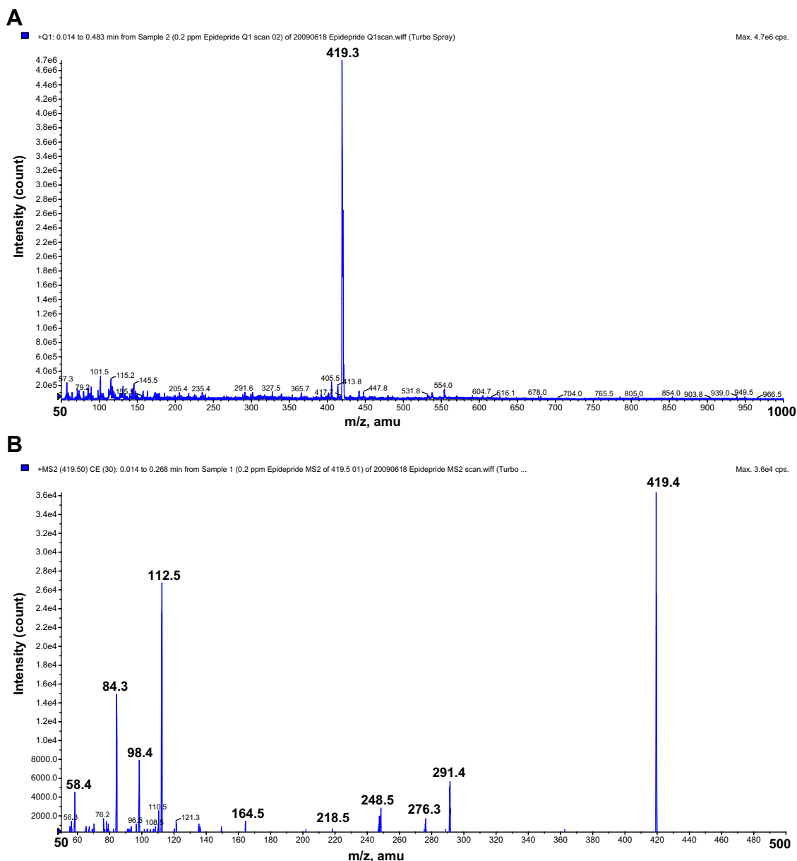
Fig. 4 – Mass spectra of epidride: (A) Q1 full scan, (B) tandem mass spectrometry from m/z 419.
