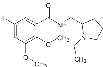
Fig. 1 – Structure of 127 I-epididepride, C 16 H 23 N 2 O 3 I – (molecular weight = 418.3).
