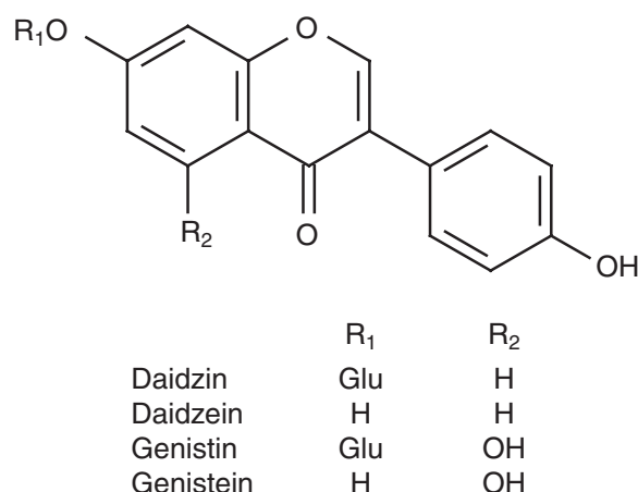
Figure 3. Structures of the studied compounds.
