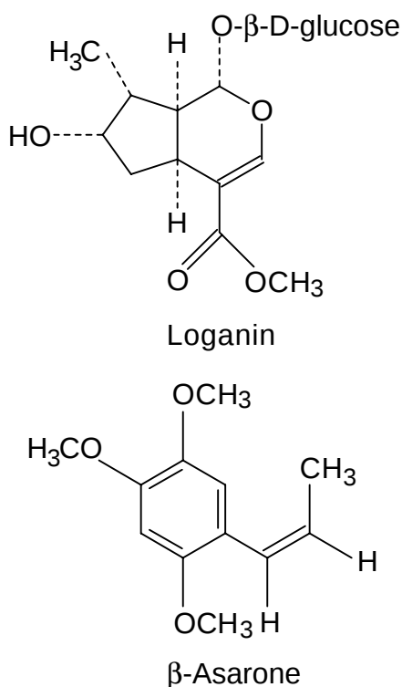
Figure 3. Chemical structure.
