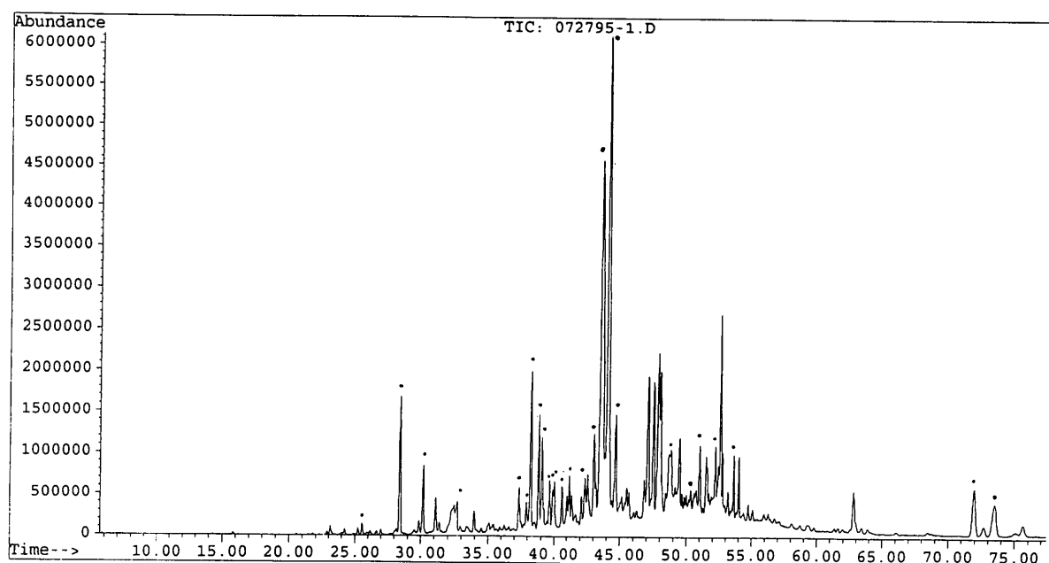
Figure 4. A typical total ion chromatogram for the extract of red cypress sawdust using SFE CO 2 extraction.
