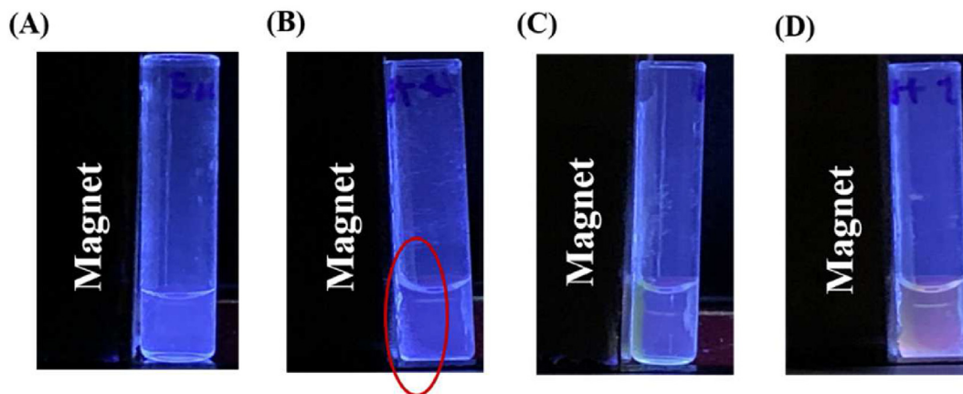
Fig. 3. Photographs of (A) \text{Eu}^{3+} only (0.05 M, 0.1 mL) and (B) our magnetic probes mixed with the same concentration of \text{Eu}^{3+} . The circulated part indicates where the magnetic conjugates are. Photographs of our magnetic probe-TC conjugates obtained (C) before and (D) after the addition of \text{Eu}^{3+} . These photographs were taken under UV light ( \lambda = 365 \text{ nm} ) in the dark.
